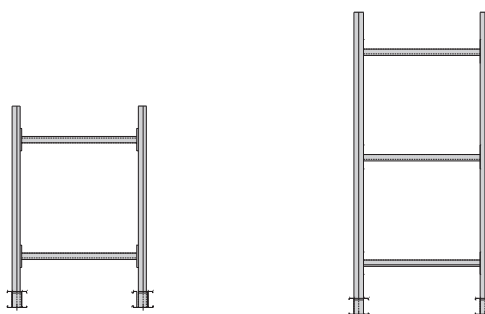
DIAGRAM E BRACING USED ON 6' - 8' UPRIGHTS
