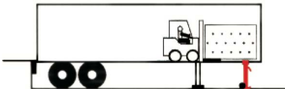
WELL-POSITIONED SUPPORT
